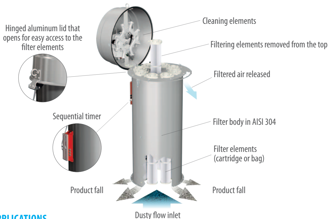
Dust aspiration from pneumatic conveying
